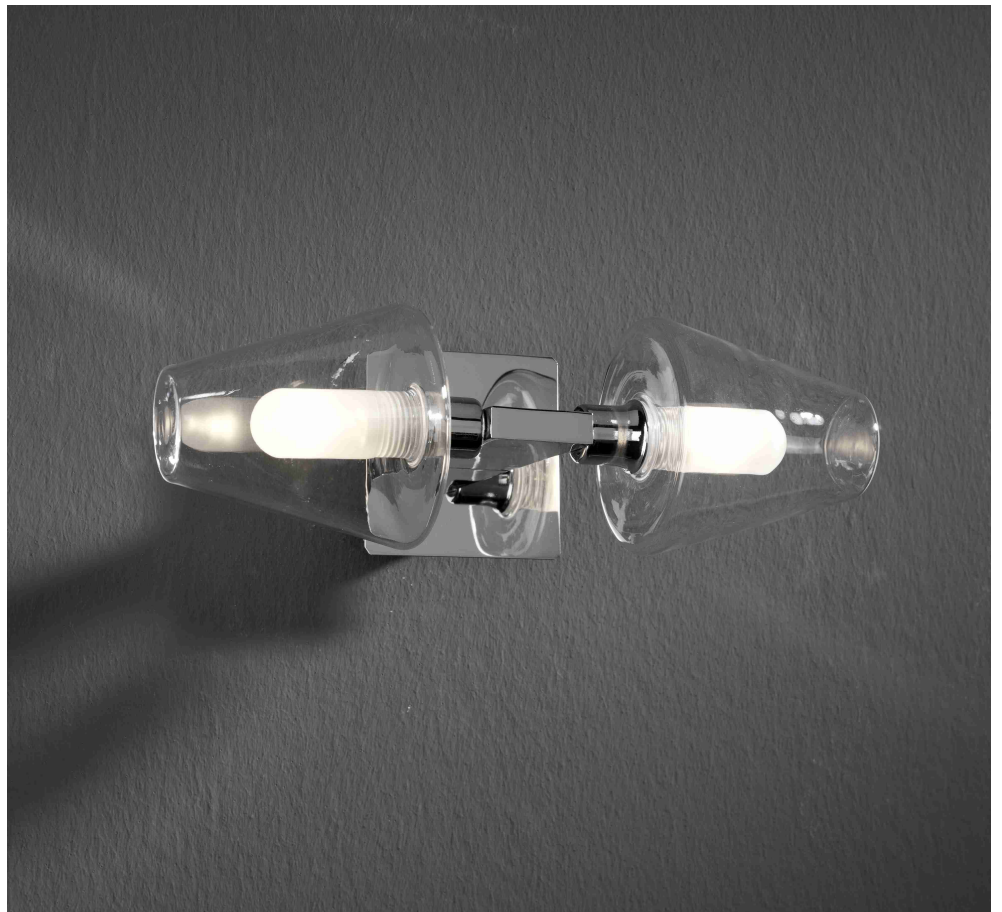
drop 246/2 2xG9. Max40w IP44 ↑9→27↗14cm Cromo Chrome
